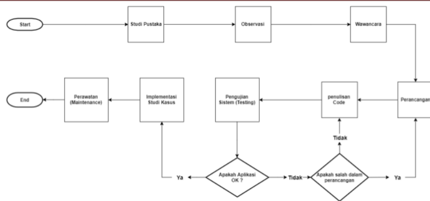
Gambar 1. Flowchart
