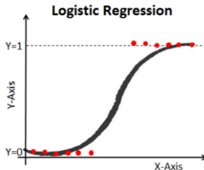
Gambar 2. Kurva Regresi logistik [15]
