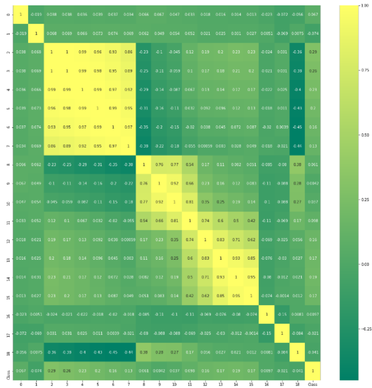
Gambar 3. Feature correlation
