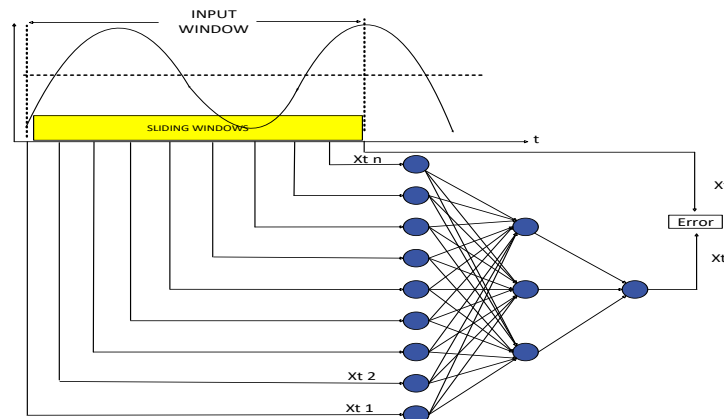
Figure 1. Windowing
