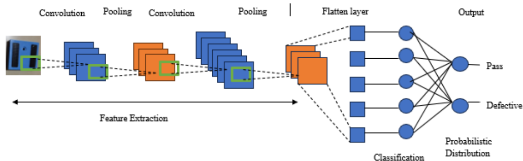
Figure 2. The workflow of the convolutional neural network algorithm
