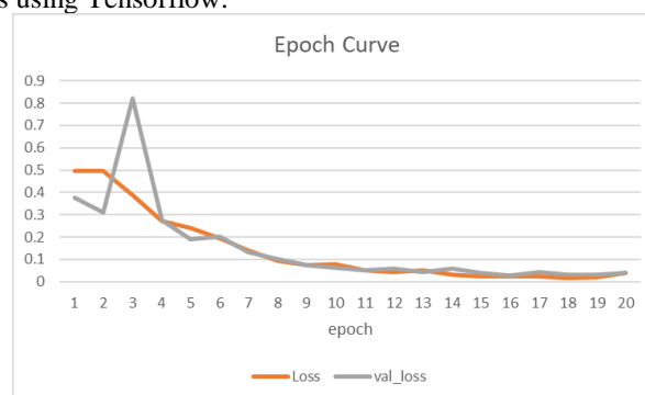
Figure 5. Loss and Val Loss in the Epoch
