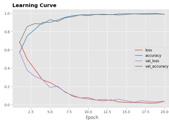
Figure 6. Learning Curve
