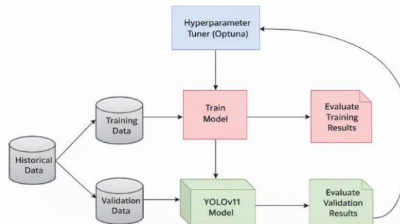
Figure 3. The Workflow of Optuna
