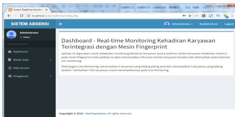
Gambar 7. Dashboard Admin
