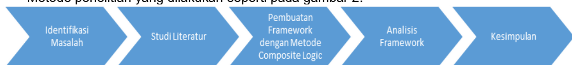
Gambar 2. Metode Penelitian
