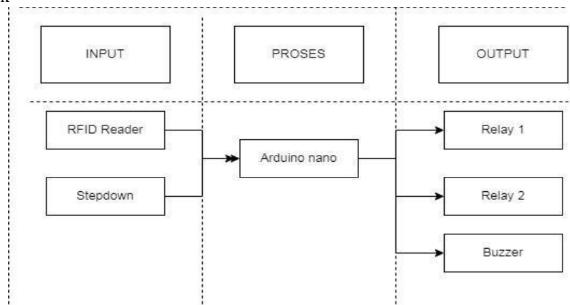
Gambar 7. Diagram Blok
