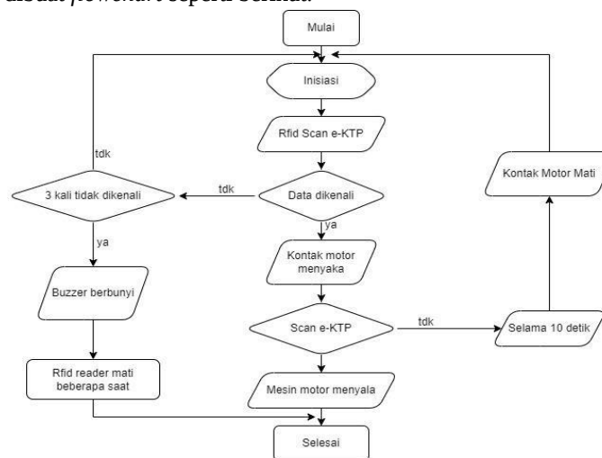
Gambar 8. Flowchart
